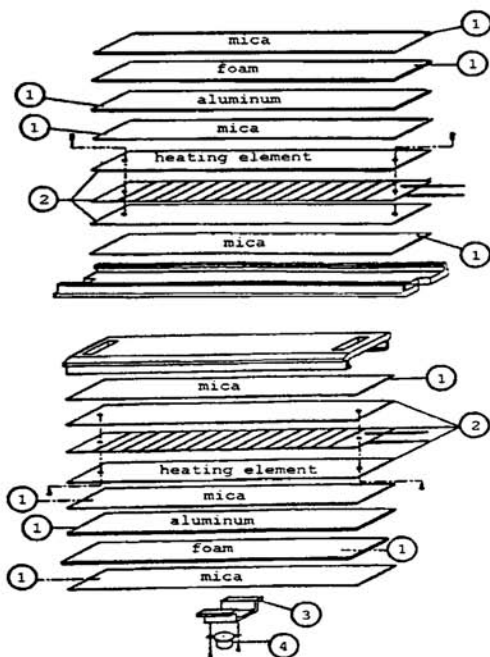
8.0 PARTS FIGURE 8.7
