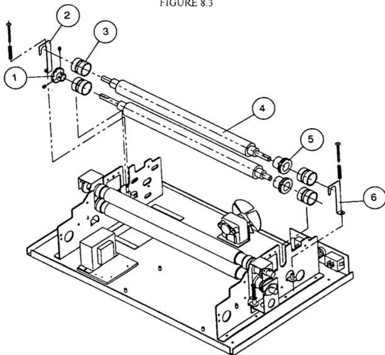
8.0 PARTS FIGURE 8.3
